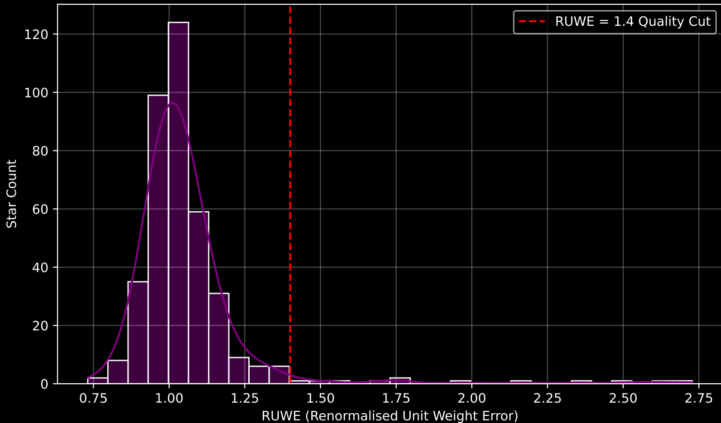
GAPOGEE DR17 Field [030+00] RUWE Distribution (n= 391)
