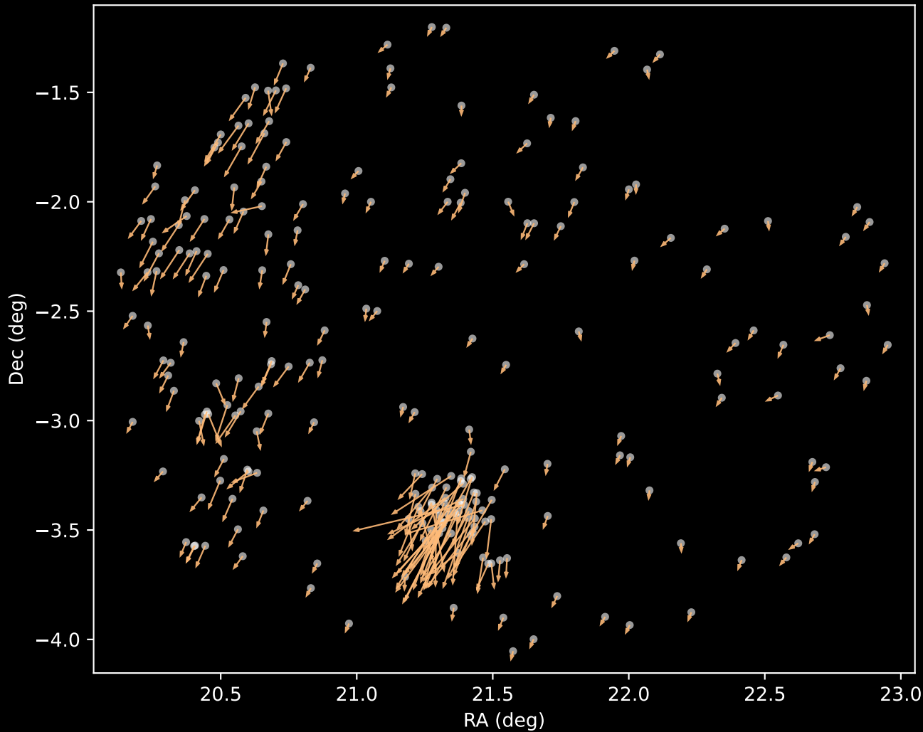
APOGEE DR17 Cluster 3 Proper Motion Vectors (n=240)
