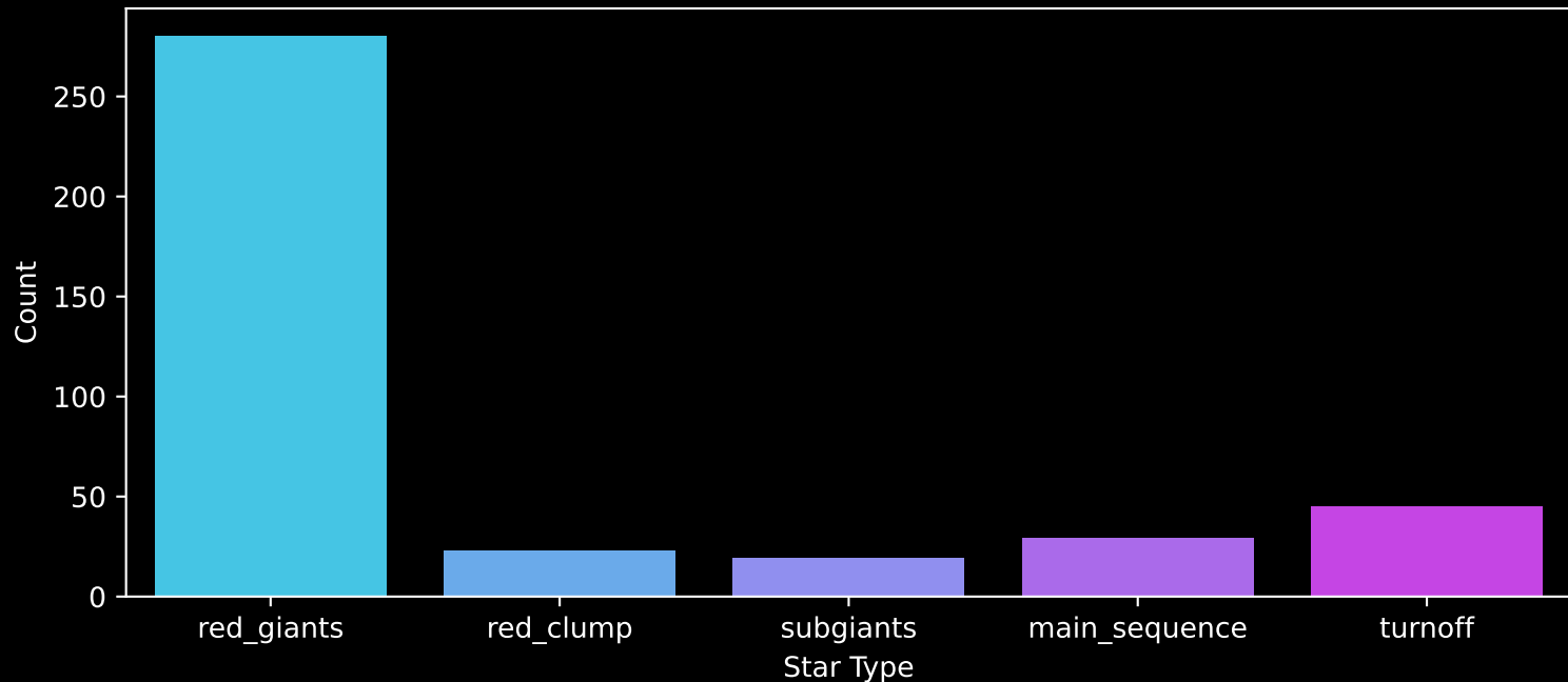
APOGEE DR17 Field: [030+00] Count plot of Star Type
