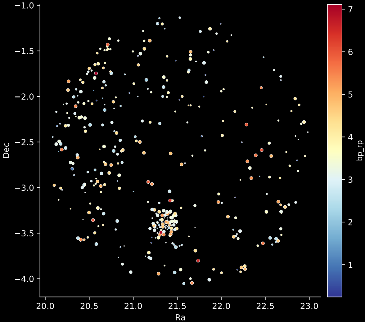
APOGEE DR17 Field: [030+00] Stars: 396
