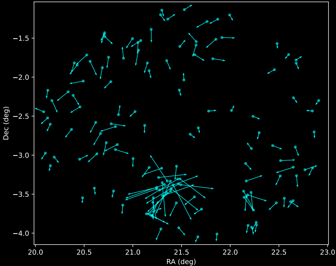
APOGEE DR17 Noise Stream Proper Motion Vectors (n=137)
