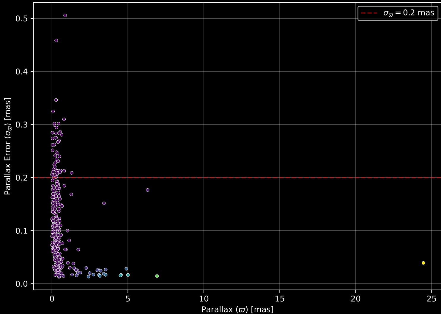
APOGEE DR17 Field: [030+00] Parallax Quality (n= 396)
