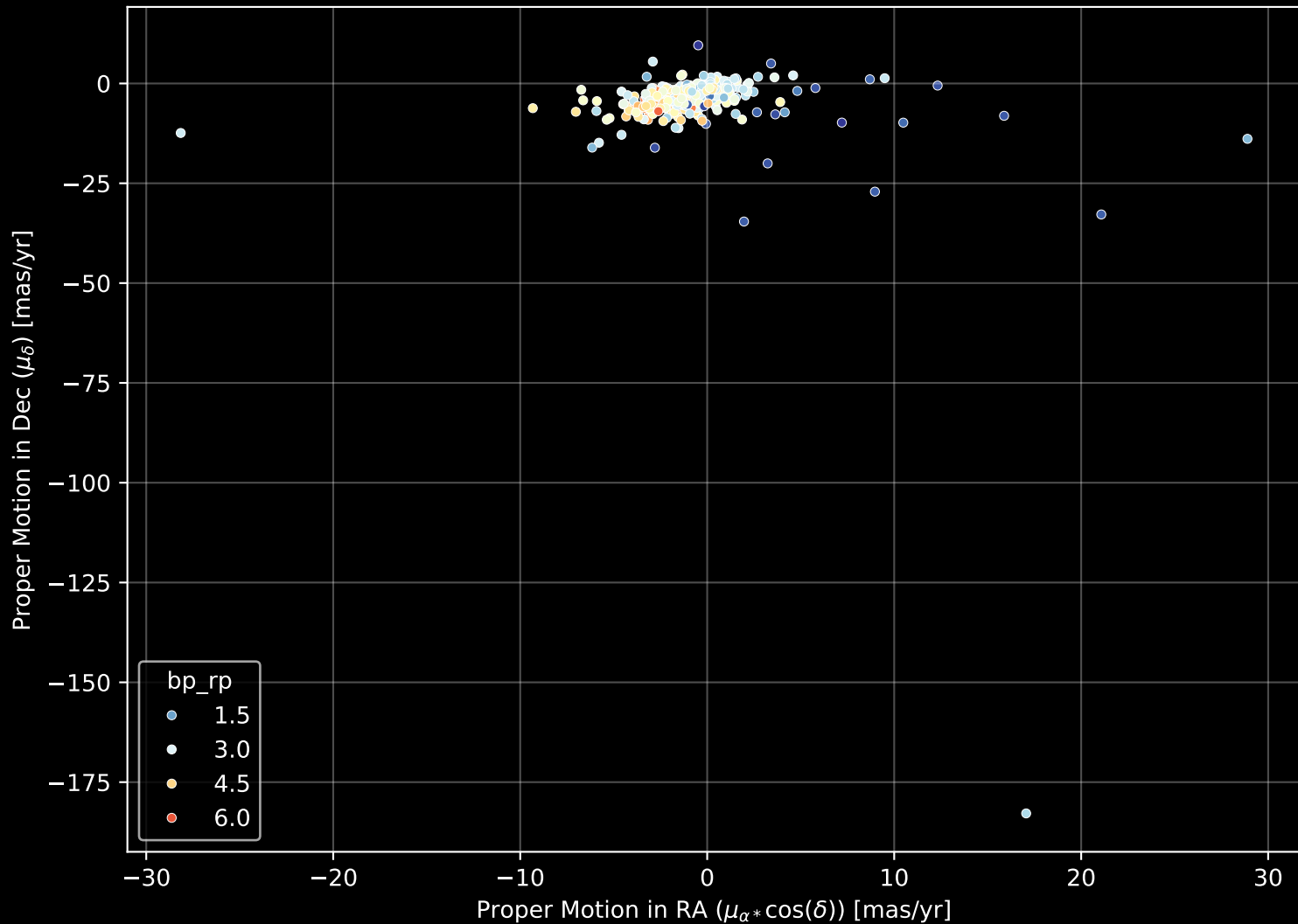
APOGEE DR17 Field: [030+00] Proper Motion Diagram (n= 396)
