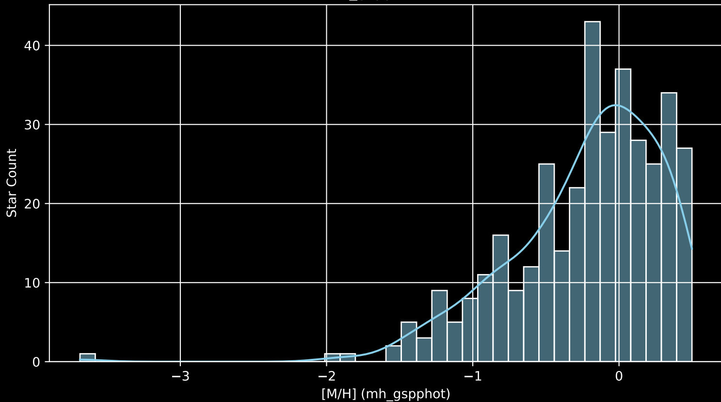
APOGEE DR17 Field: [030+00 [M/H] (mh_gspphot) (n= 367)
